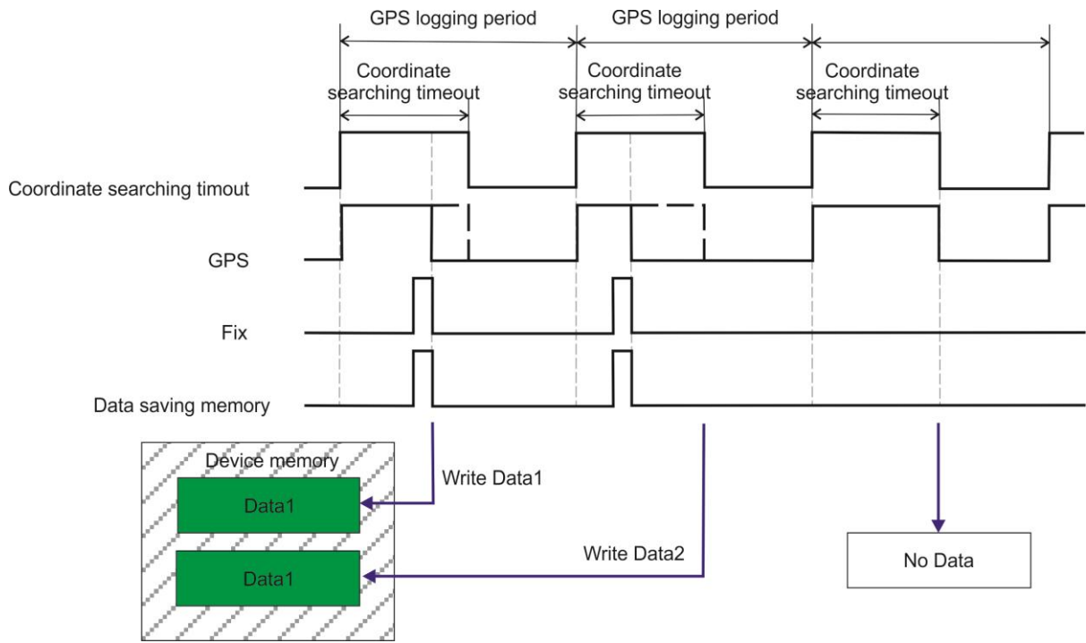
Periodical data saving, when data is saved after coordinate is found ( When location available only )
