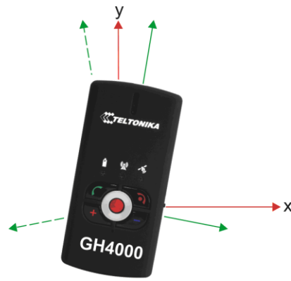
Position changed less than 68^\circ degrees. PreAlarm is not activated.
