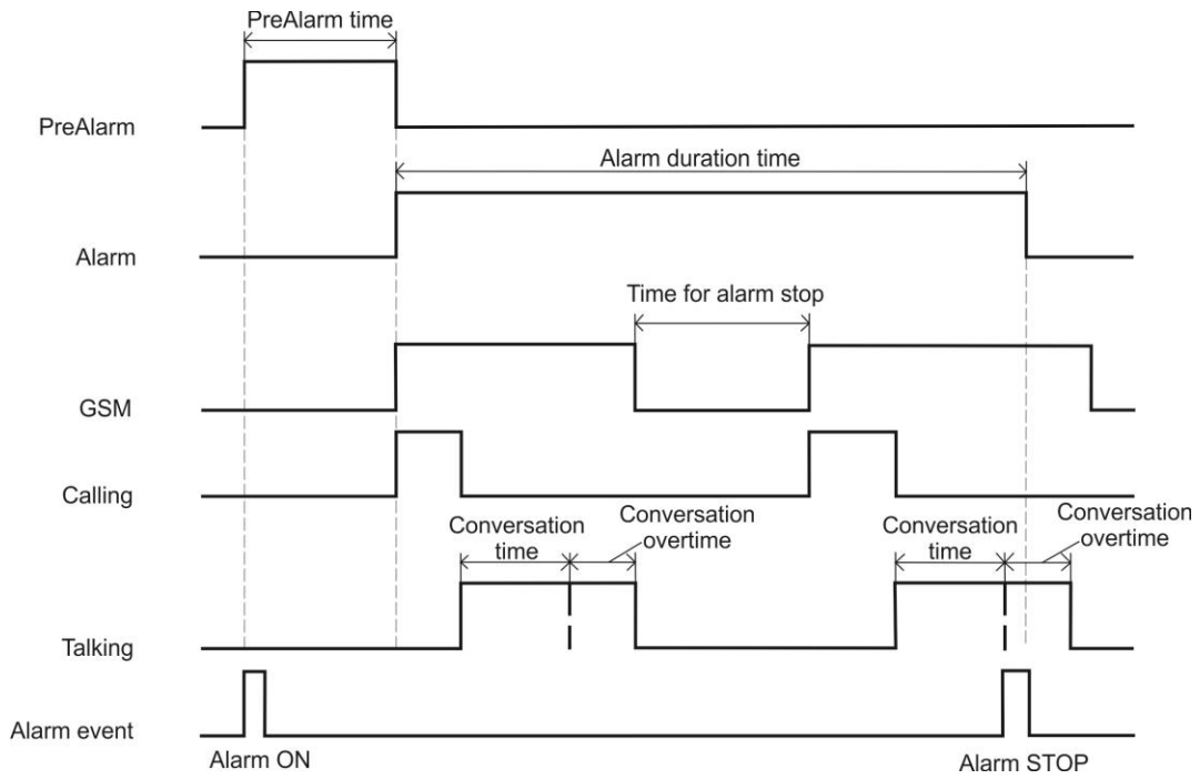
Call method
