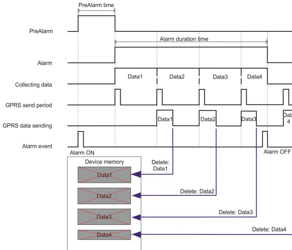
GPRS method
