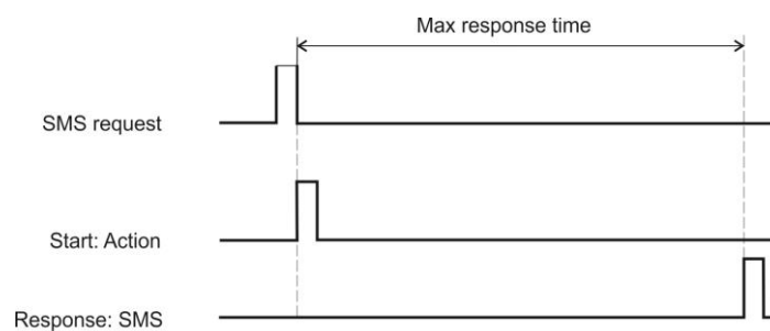
Operation of SMS request and respond
